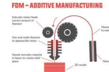
FDM Printing
